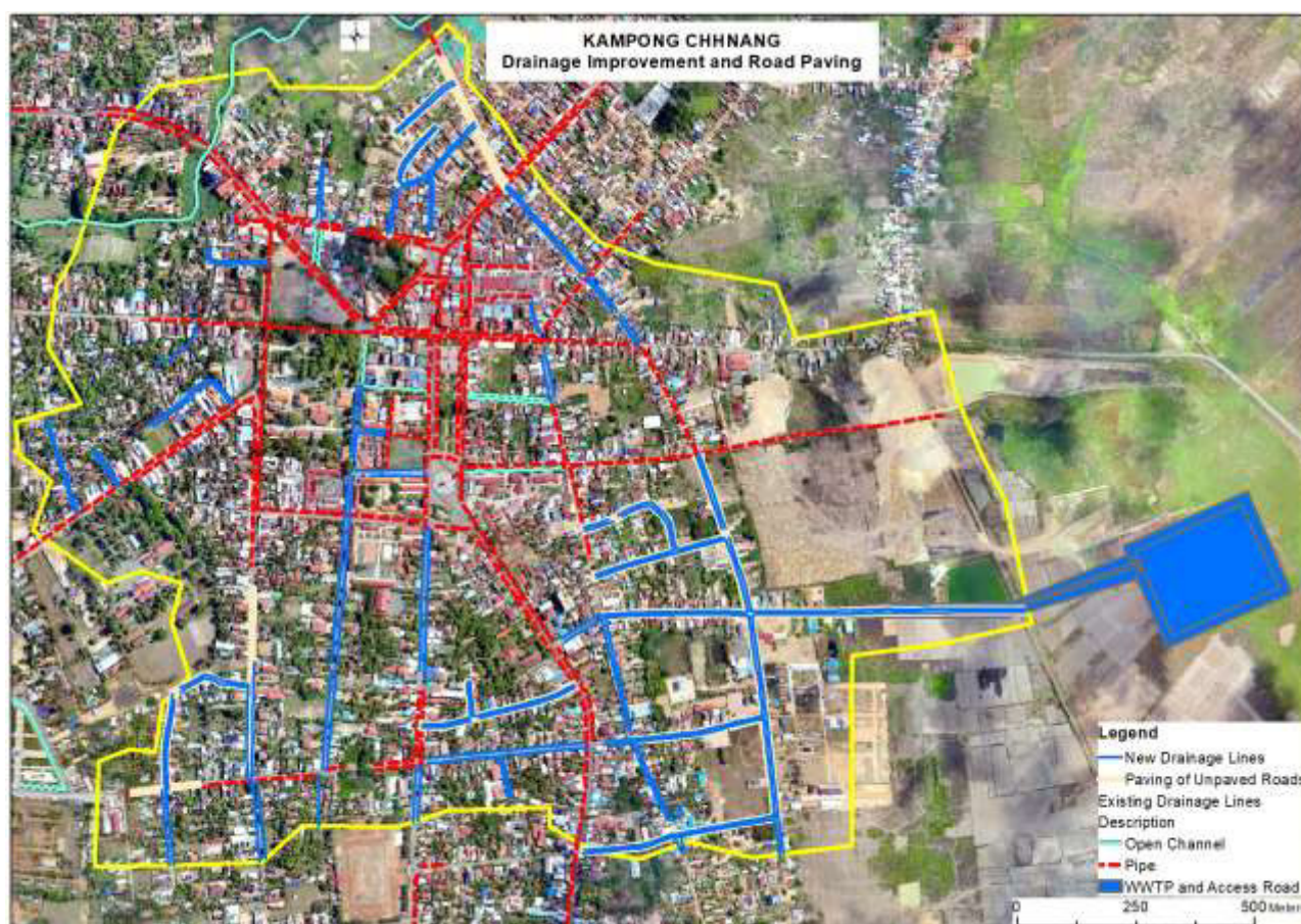
Figure 8 Drainage improvements and road paving location
